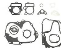
948527 Junta Motor Completa BIZ 100 98-05/DREAM - BHD
